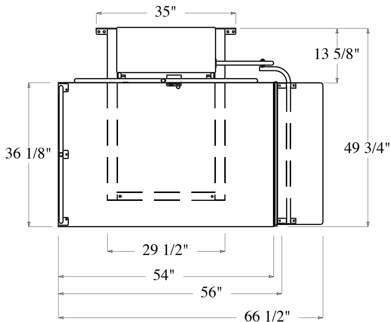
PL-50 TOP VIEW: 36X54 INCH 90 DEGREE EXIT PLATFORM
