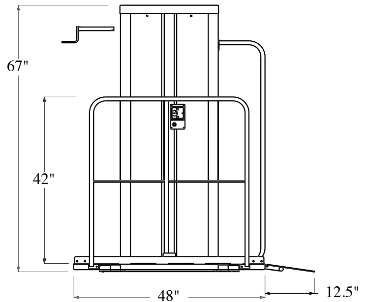
PL-50 FRONT VIEW: 32X48 INCH PLATFORM
